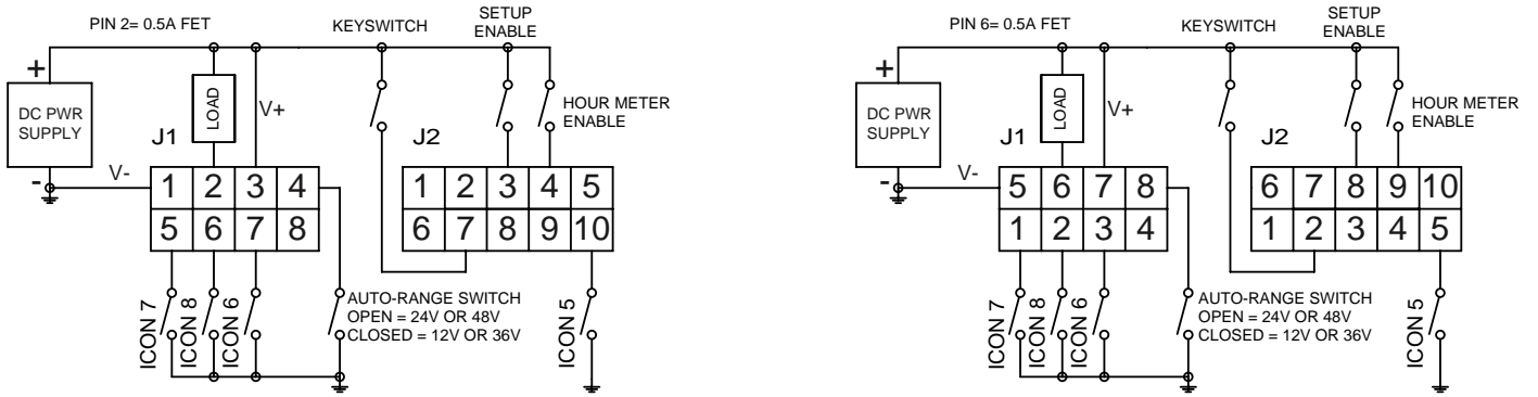
BDI (with auto-range switch)
